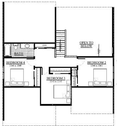
SECOND FLOOR LAYOUT
