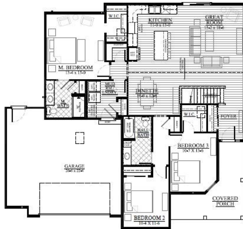
FIRST FLOOR LAYOUT
