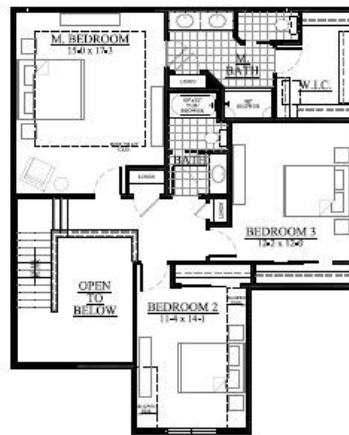
SECOND FLOOR LAYOUT
