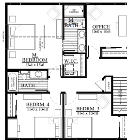
SECOND FLOOR LAYOUT
