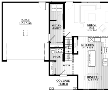
FIRST FLOOR LAYOUT
